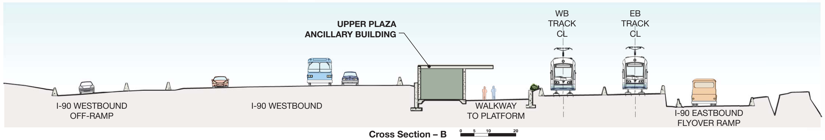
Station Site Section/Cross Sections
