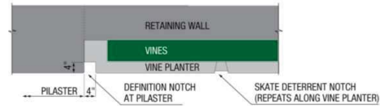
PLAN SECTION: VINE PLANTER NOTCH AT PILASTER
