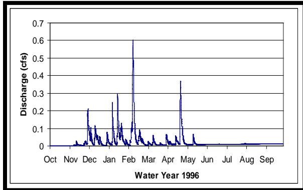
Figure F.4. Runoff from 10-Acre Forested Site.
