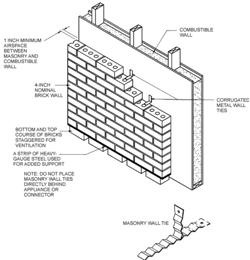
FIGURE G2409.2(2) [308.2(2)] WALL PROTECTOR CLEARANCE REDUCTION SYSTEM
