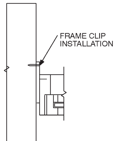
APPLY FRAME CLIP TO WINDOW OR DOOR IN ACCORDANCE WITH PUBLISHED MANUFACTURER'S RECOMMENDATIONS.
