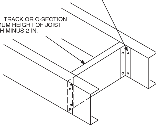
SOLID BLOCKING
