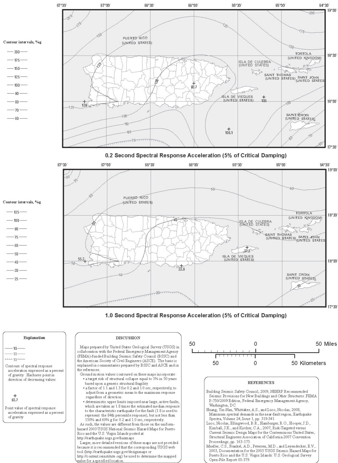
FIGURE 1613.3.1(6) RISK-TARGETED MAXIMUM CONSIDERED EARTHQUAKE ( MCE_R ) GROUND MOTION RESPONSE ACCELERATIONS FOR PUERTO RICO AND THE UNITED STATES VIRGIN ISLANDS OF 0.2- AND 1-SECOND SPECTRAL RESPONSE ACCELERATION (5% OF CRITICAL DAMPING), SITE CLASS B
