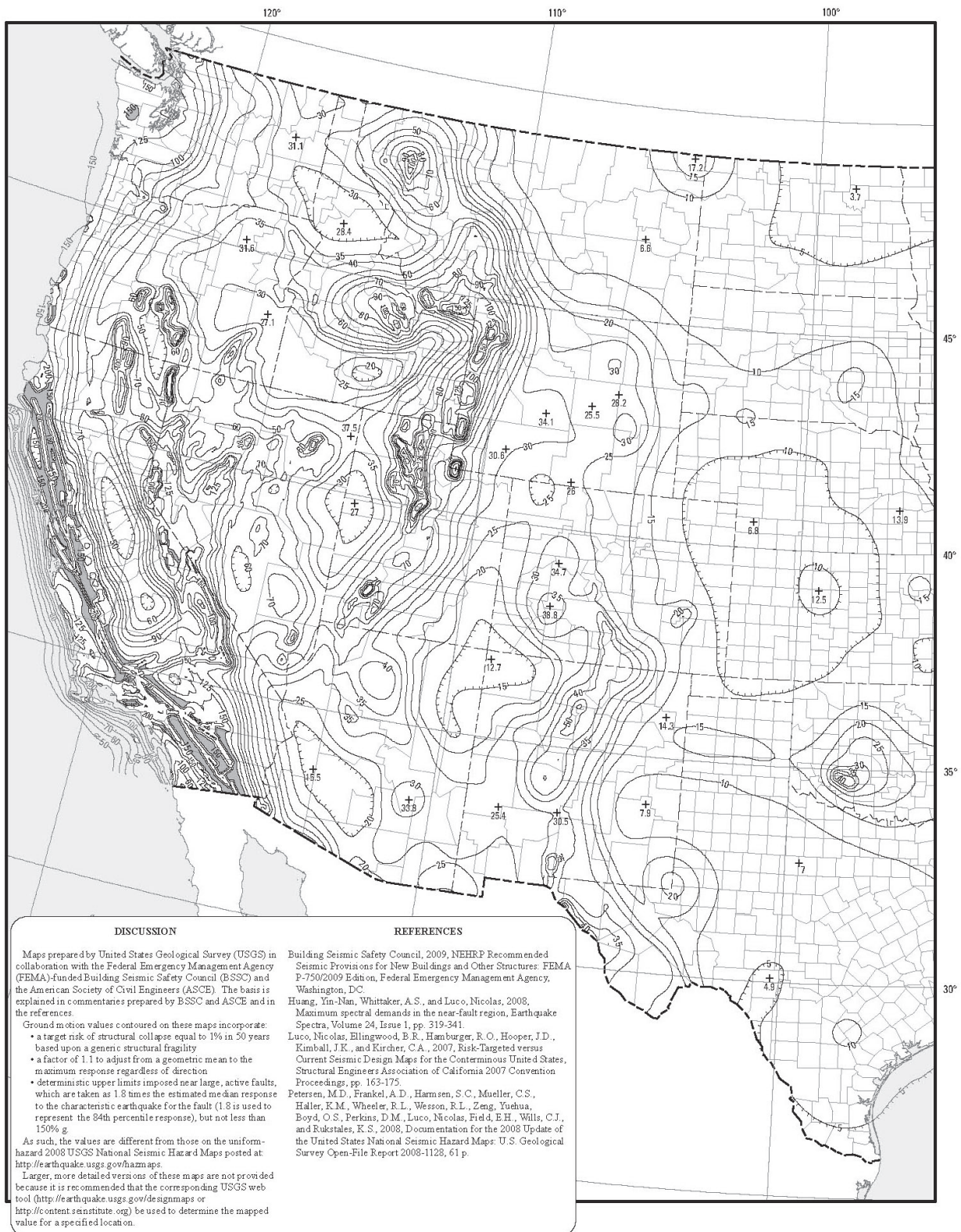
FIGURE 1613.3.1(1) RISK-TARGETED MAXIMUM CONSIDERED EARTHQUAKE ( MCE_B ) GROUND MOTION RESPONSE ACCELERATIONS FOR THE CONTERMINOUS UNITED STATES OF 0.2-SECOND SPECTRAL RESPONSE ACCELERATION (5% OF CRITICAL DAMPING), SITE CLASS B
