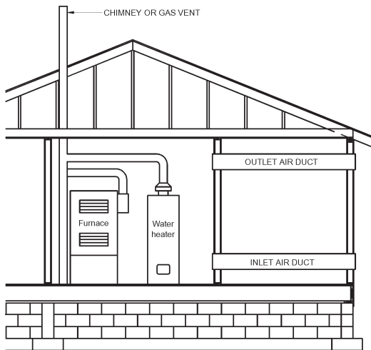
FIGURE 304.6.1(3) ALL AIR FROM OUTDOORS (see Section 304.6.1)
