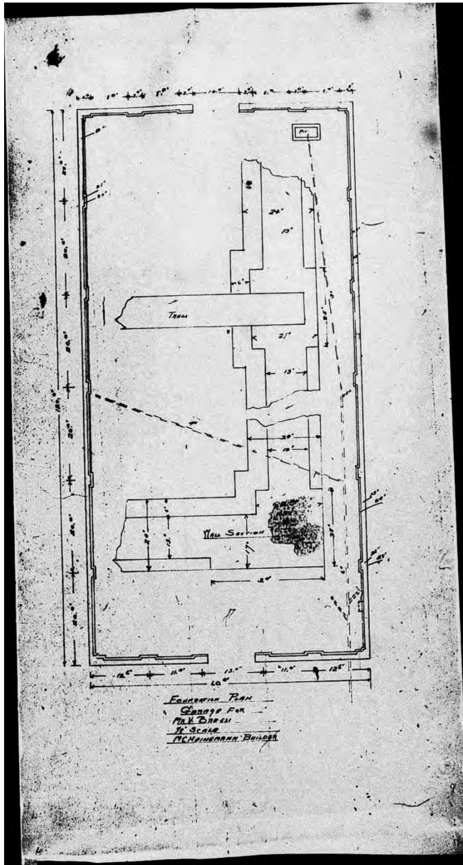
Figure 19: Foundation plan, Bressi Garage. March 1923. M.C. Heinemann, Builder. Courtesy Seattle Department of Planning and Development Microfilm Library.
