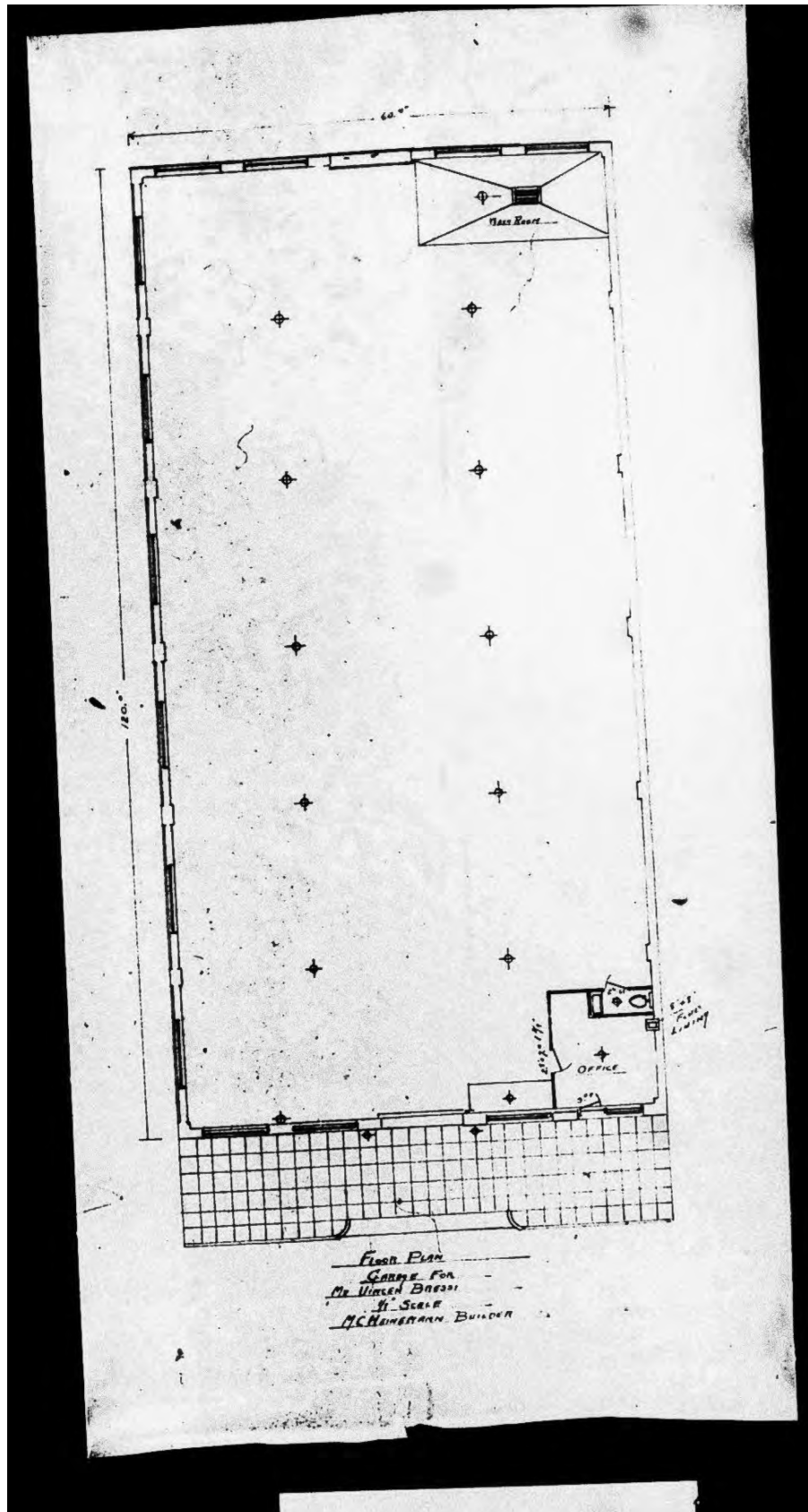
Figure 20: Floor plan, Bressi Garage. March 1923. M.C. Heinemann, Builder. Courtesy Seattle Department of Planning and Development Microfilm Library.
