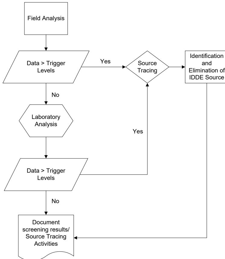
Figure B-1 IDDE Field Screening Flow Chart
