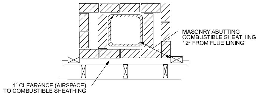
FIGURE 2113.19 ILLUSTRATION OF EXCEPTION THREE CHIMNEY CLEARANCE PROVISION
