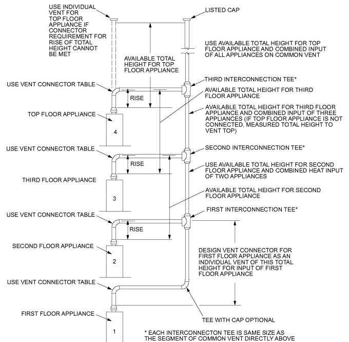
FIGURE B-14 MULTISTORY VENT SYSTEMS
