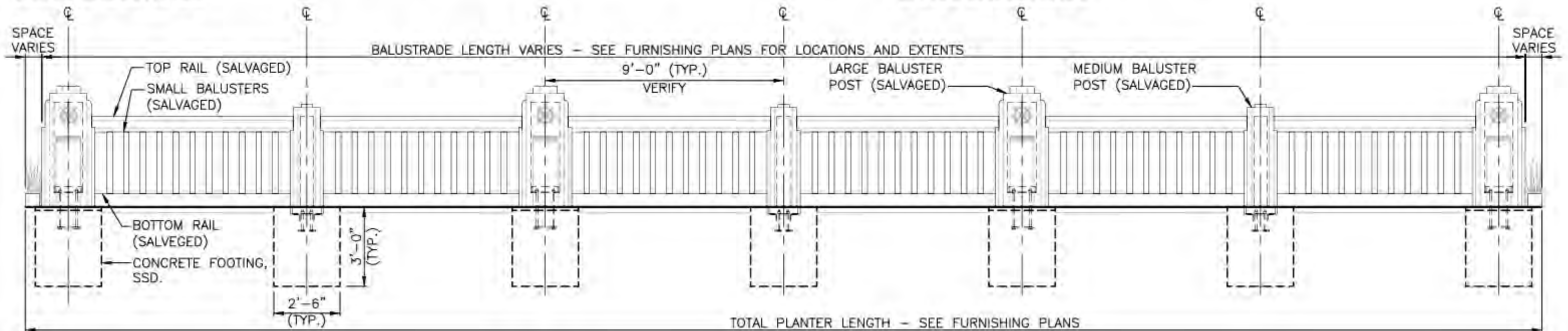
BALUSTRADE TYPICAL ELEVATION
