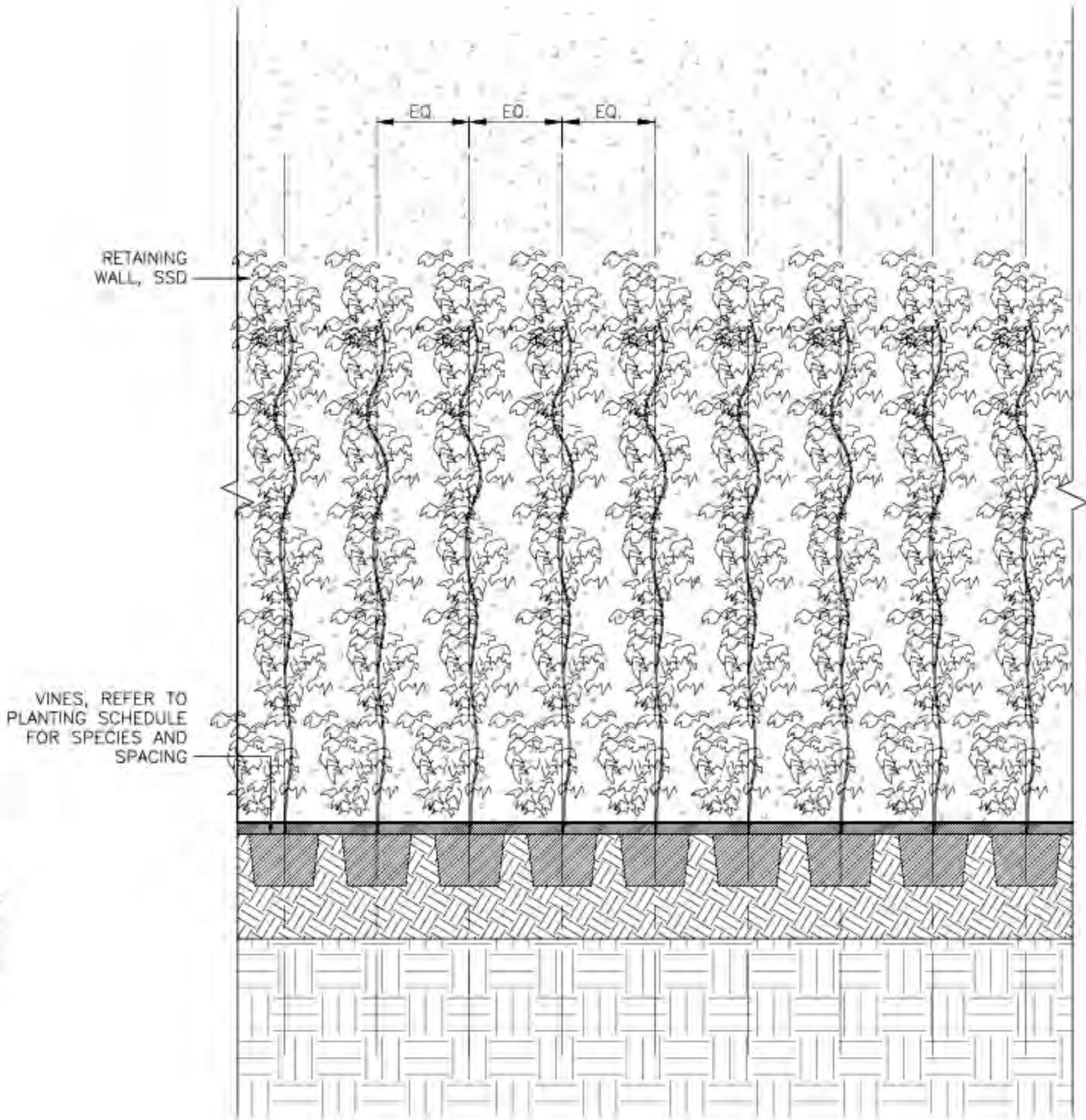
RETAINING WALL D ELEVATION
