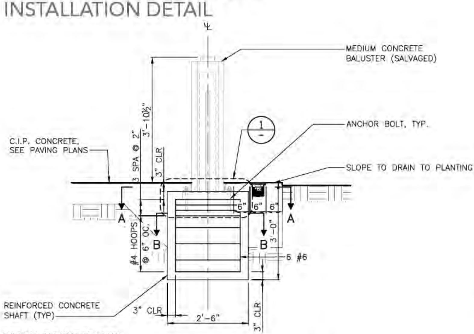
SMALL BALUSTRADE
