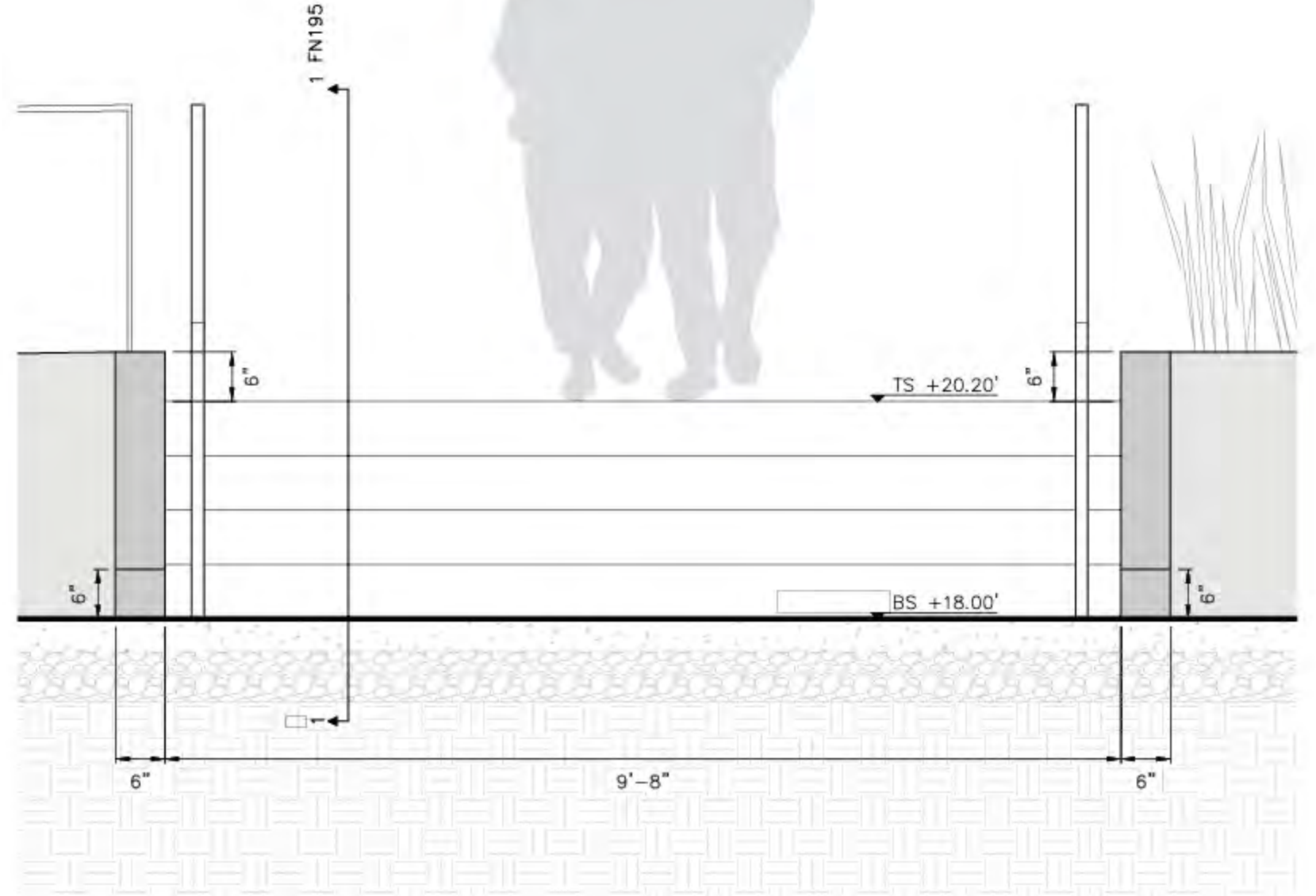
STAIR + RAILING ELEVATION
