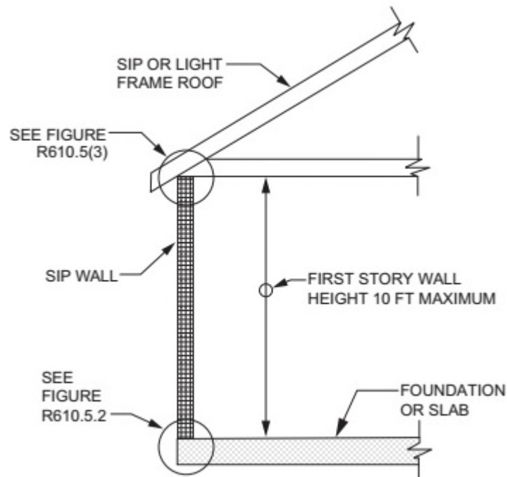
FIGURE R610.5(1) MAXIMUM ALLOWABLE HEIGHT OF SIP WALLS
