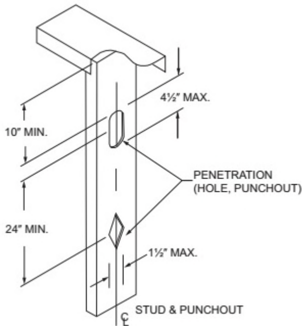
FIGURE R603.2.6.1 WALL STUD WEB HOLES
