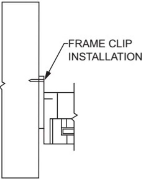
FIGURE R609.7.2(2) FRAME CLIP
