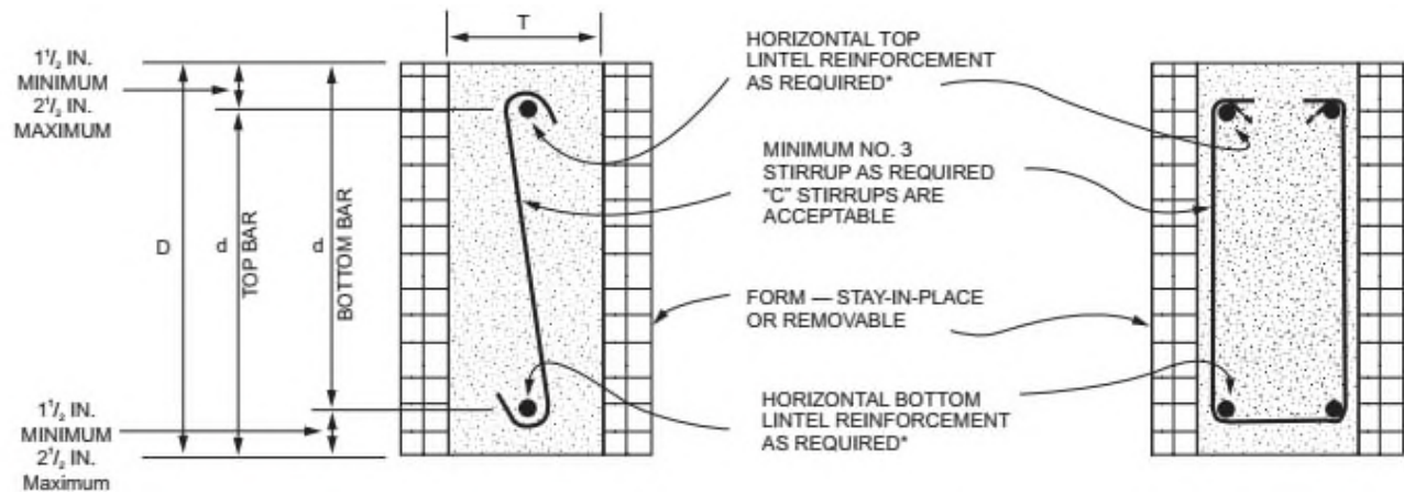
FIGURE R608.8(2) LINTEL FOR FLAT WALLS
