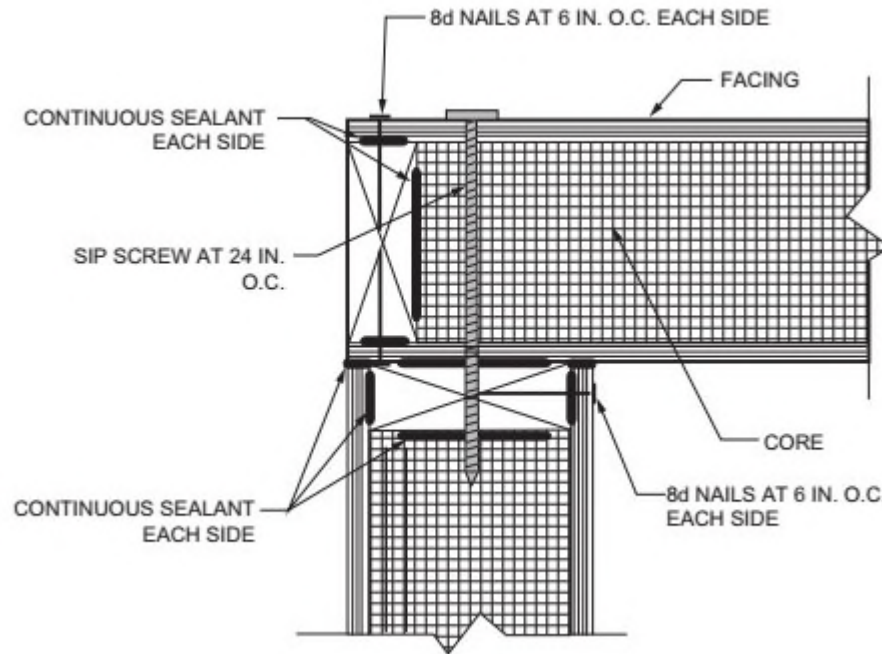
FIGURE R610.5.4 SIP CORNER FRAMING DETAIL
