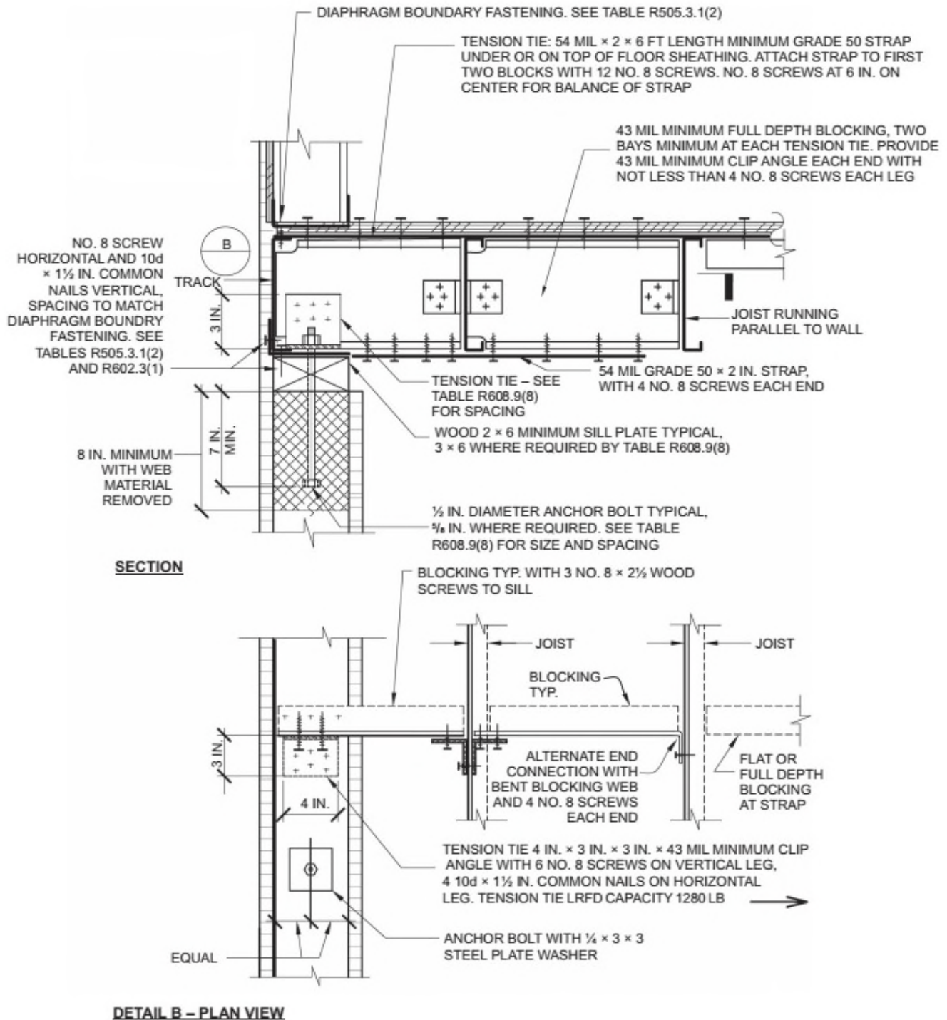
FIGURE R608.9(8) COLD-FORMED STEEL FLOOR TO TOP OF CONCRETE WALL, FRAMING PARALLEL
