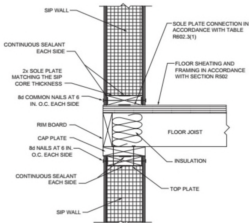
FIGURE R610.5(4) SIP WALL-TO-WALL PLATFORM FRAME CONNECTION
