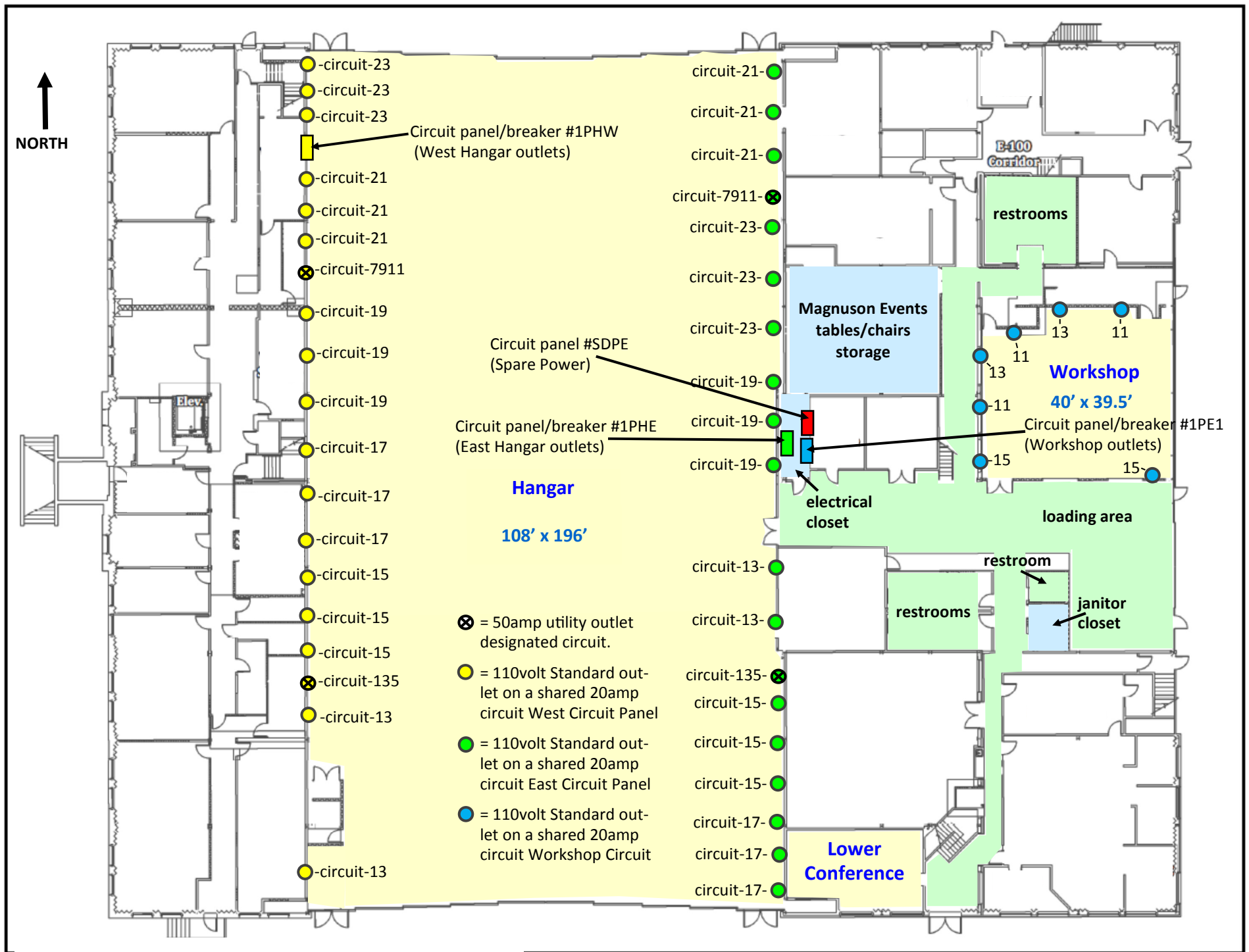
Building 30—first floor Electricity Map
