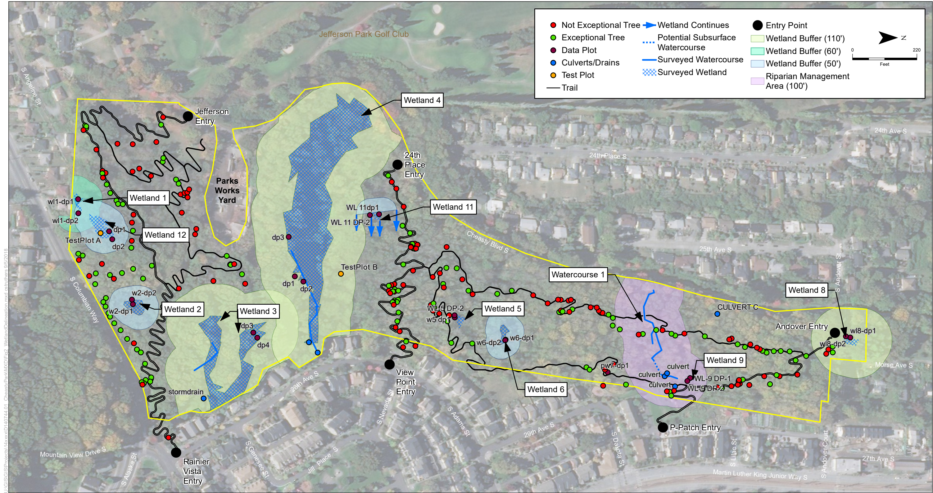
Figure 2 Wetland Delineation and Trail Design
