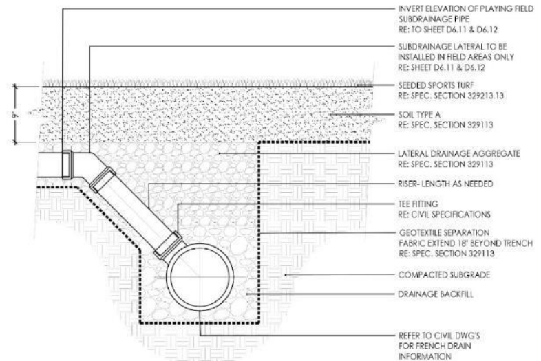
Lateral to Collector Sub-Drainage
