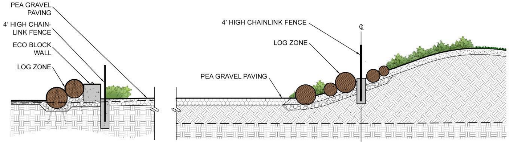
Edge Conditions of Off-Leash Area
