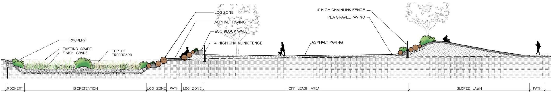
Section of Berm, Off-Leash Area, and Bioretention; Looking West
