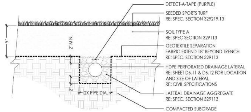
Sports Lawn Soil with Lateral
