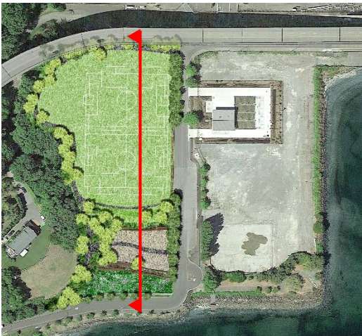
Section of Berm, Off-Leash Area, and Bioretention; Looking West
