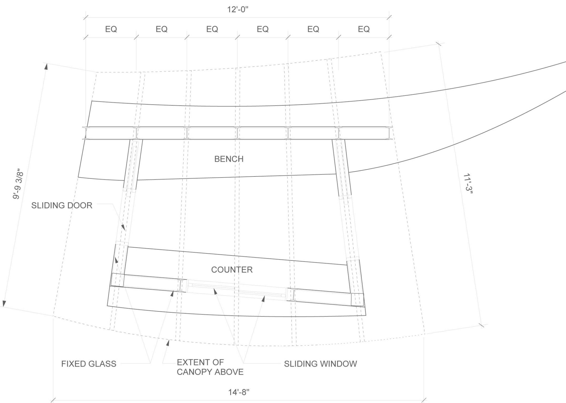
PLAN
