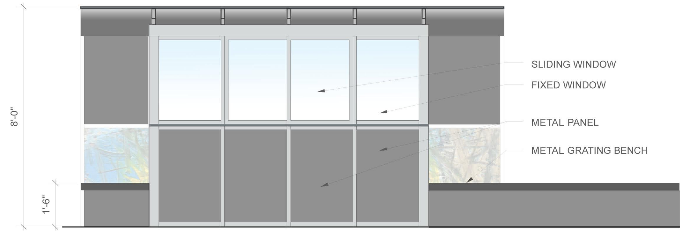
SOUTH ELEVATION
