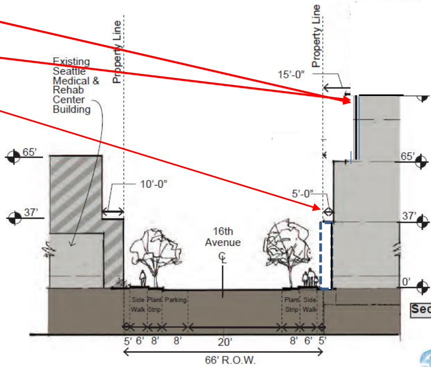
-REVISED SECTION K-K 1
