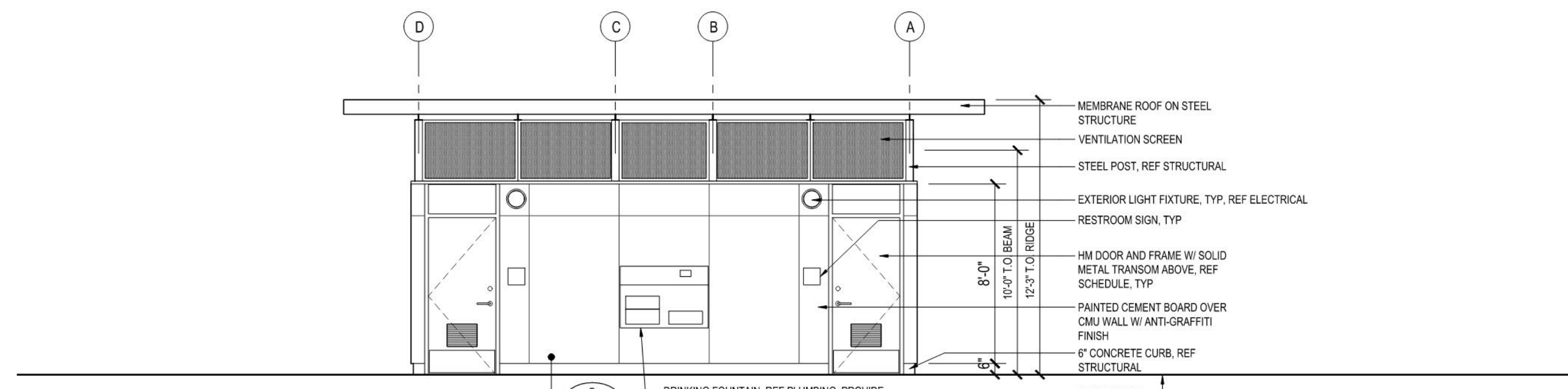
3 ELEVATION 1/4" = 1'-0"
