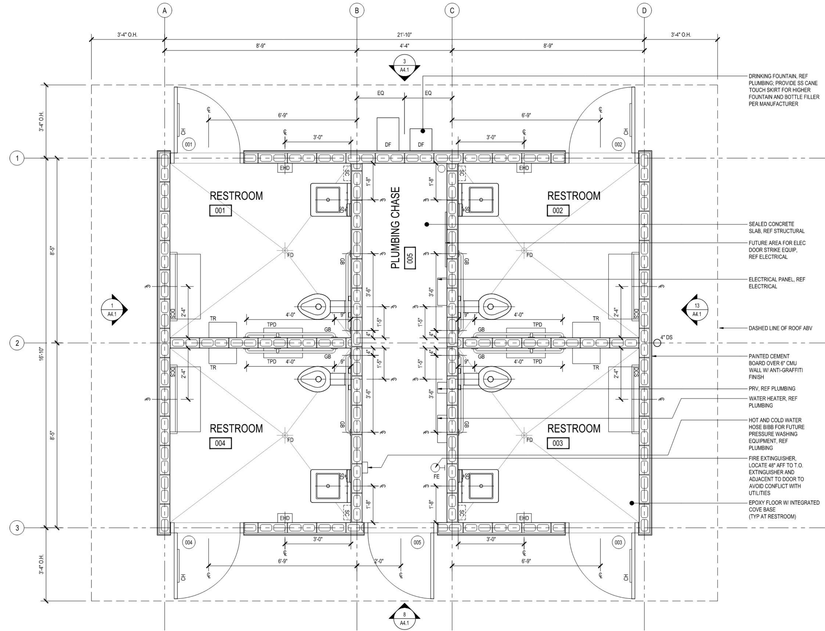
12 RESTROOM FLOOR PLAN
